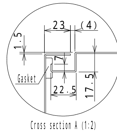
Cross section A (1:2)
